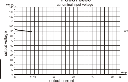
load diagram PS3U75090 at nominal input voltage
