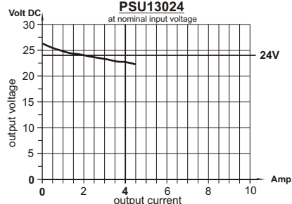
load diagram PSU13024
