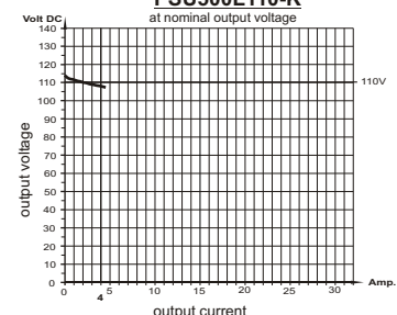
load diagram PSU500L110-K at nominal output voltage
