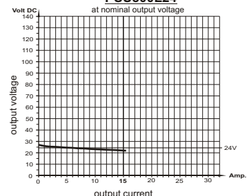
load diagram PSU500L24 at nominal output voltage
