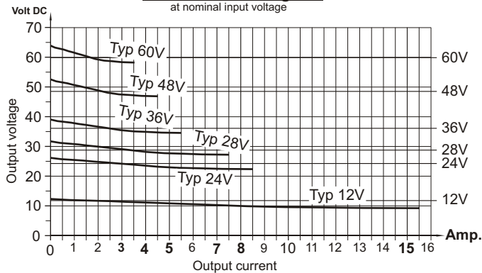
Load current diagram at nominal input voltage
