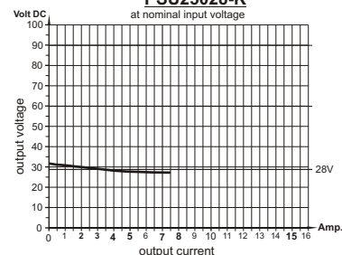
load diagram PSU25028-K at nominal input voltage
