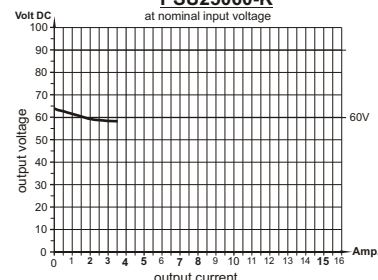
load diagram PSU25060-K at nominal input voltage
