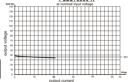
load diagram PS2U75036-K at nominal input voltage
