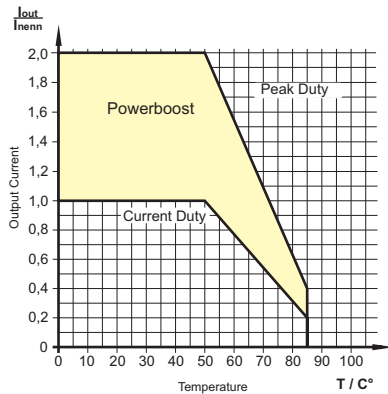
Load Current Diagram at nominal Input
