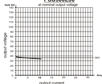
load diagram PSU500L36 at nominal output voltage
