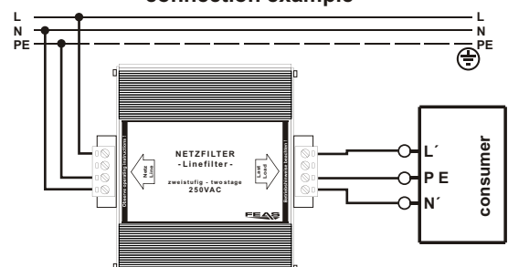
connection example
