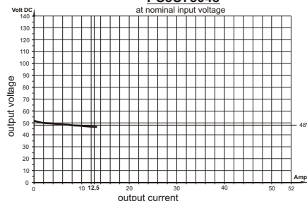
load diagram PS3U75048 at nominal input voltage
