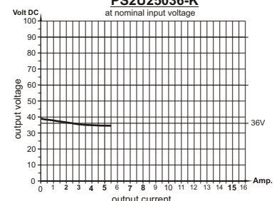
load diagram PS2U25036-K at nominal input voltage
