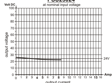
load diagram PSU25024 at nominal input voltage
