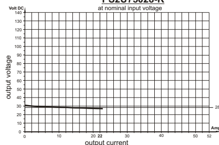
load diagram PS2U75028-K at nominal input voltage
