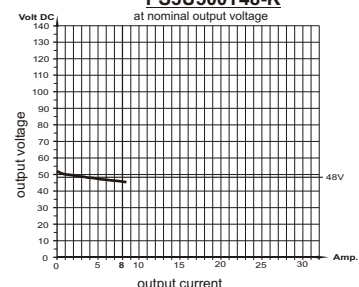
load diagram PS3U500T48-K at nominal output voltage
