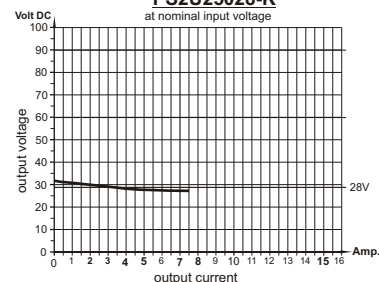
load diagram PS2U25028-K at nominal input voltage
