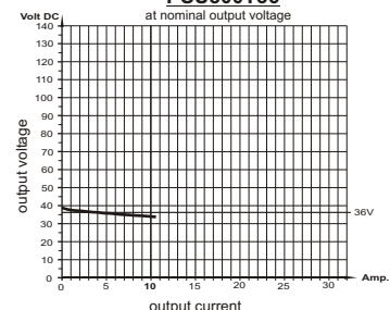
load diagram PSU500T36 at nominal output voltage
