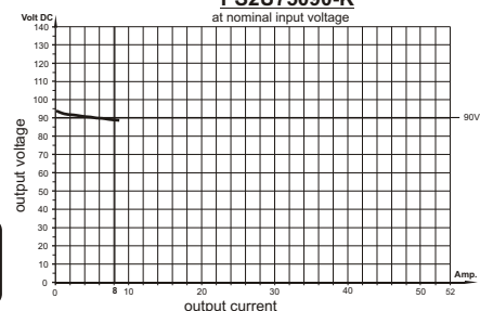
load diagram PS2U75090-K at nominal input voltage
