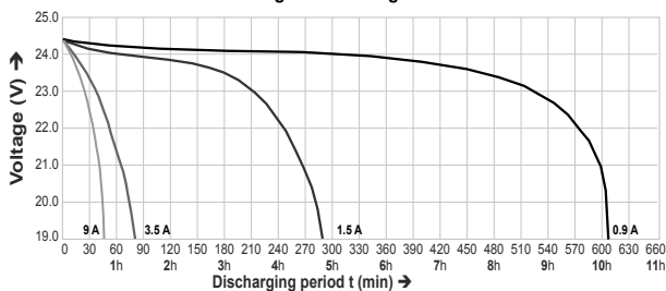
Discharge current diagram at 25°C
