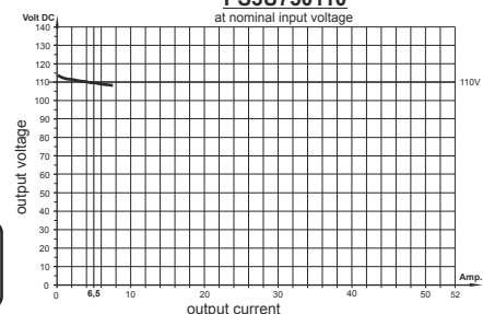
load diagram PS3U750110 at nominal input voltage
