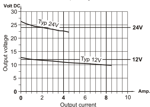
Load-current diagram at nominal input voltage
