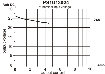
load diagram PS1U13024 at nominal input voltage
