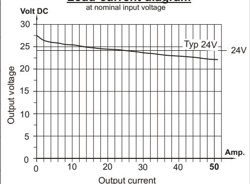
Load-current diagram at nominal input voltage
