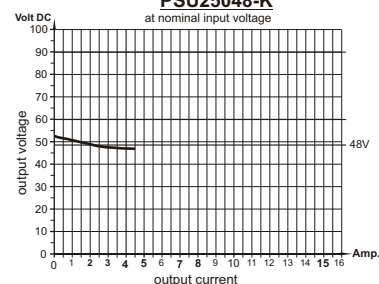
load diagram PSU25048-K at nominal input voltage
