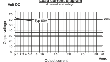
Load current diagram at nominal input voltage
