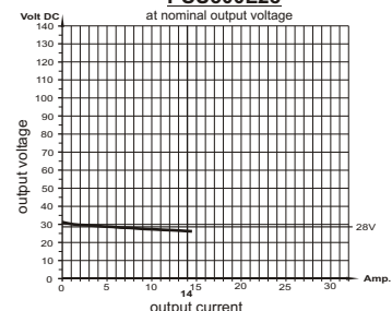
load diagram PSU500L28 at nominal output voltage
